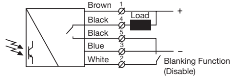
SGR 14 (load as NPN)
